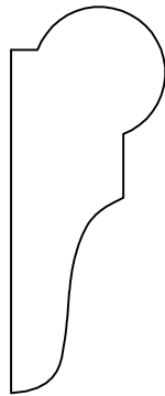
BWP-3902 3/4" X 1 13/16"
