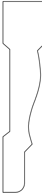
BWP-2005 11/16" x 3 1/4"
