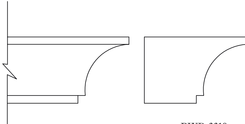
BWP-3310 1 1/8" x 1 3/4"
