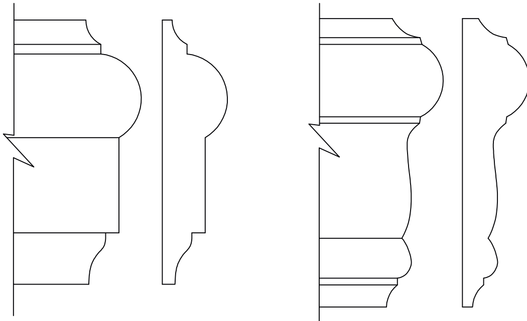
BWP-4005 11/16" x 3"
