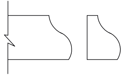
BWP-1501 9/16" x 3/4"
