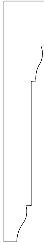
BWP-2023 11/16" x 2 1/2"
