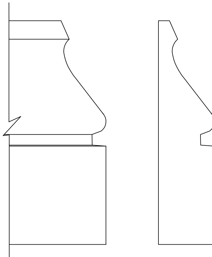
BWP-1514 15/16" x 3 3/4"
