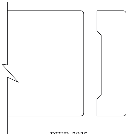
BWP-2035 5/8" x 2 1/4" 1/16" RADIUS
