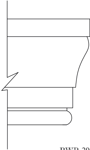
BWP-2022 11/16" x 2 1/4"
