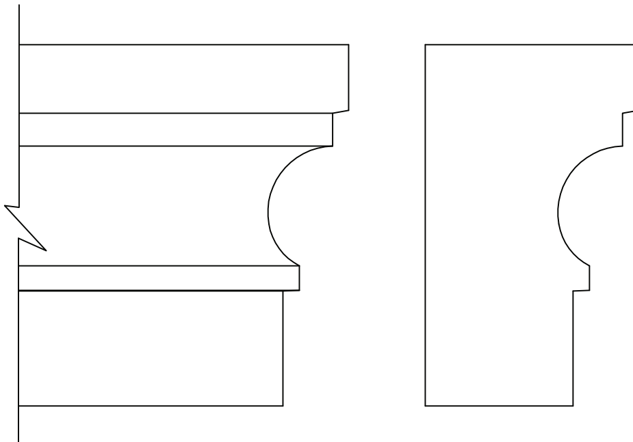
BWP-8003 1 5/8" x 2 3/4"
