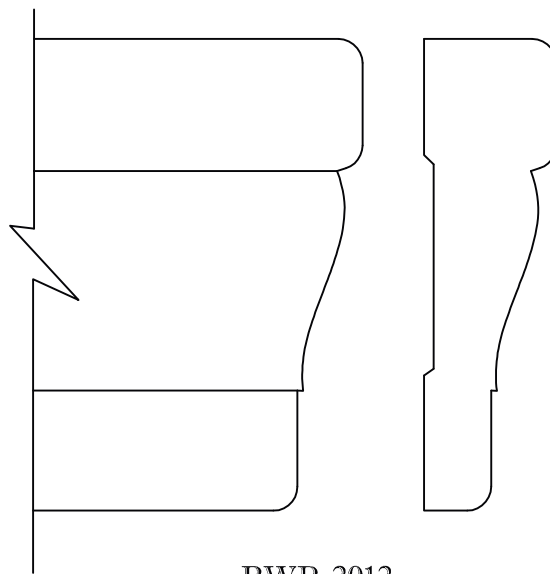
BWP-2012 11/16" x 2 1/2"
