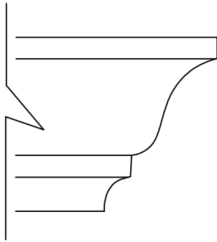
BWP-3001 9/16" x 1 5/8"
