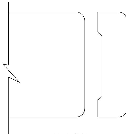
BWP-2034 5/8" x 2 1/4" 1/8" RADIUS
