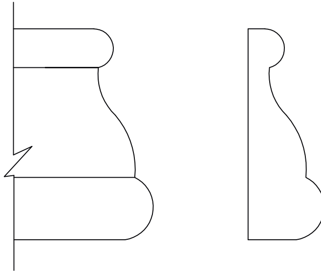
BWP-1513 13/16" x 2 1/4"
