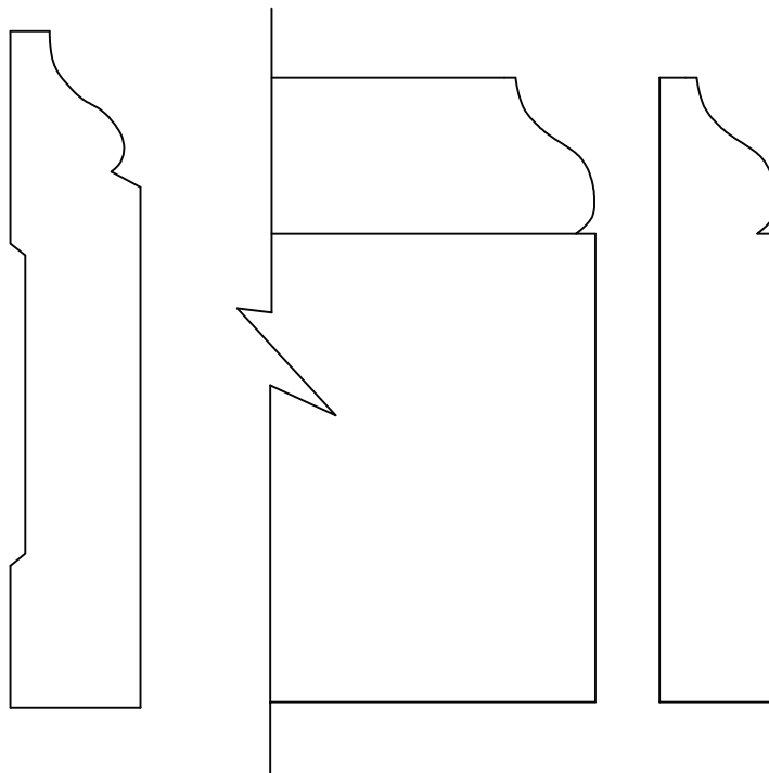
BWP-1002 9/16" x 3"
